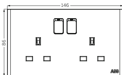
Ø3 Dimensions for 2gang frames
