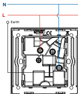
O20 1G 15 A switched socket outlet
