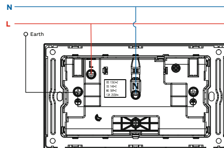
O18 2G 13 A switched socket outlet
