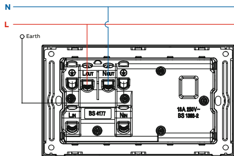
O13 Cooker switch unit
