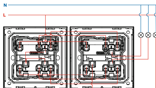
○7 3G 2W switch
