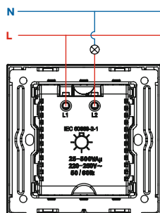
O33 Rotary dimmer
