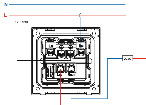
O12 1G 1W switch 32A/45A DP
