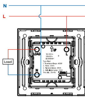
O30 Electronic Card Switch
