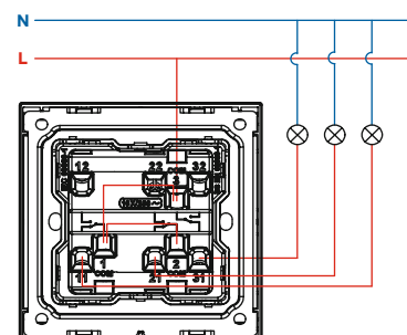
○3 3G 1W switch
