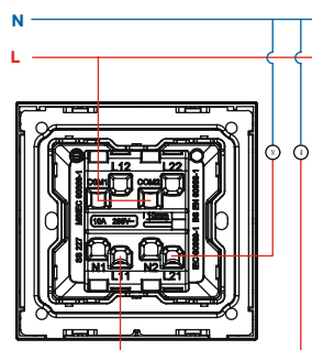
O29 Blind Control Switch
