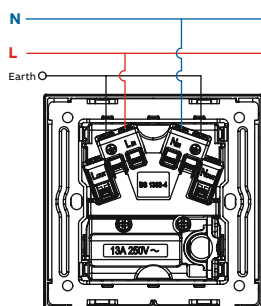
O37 Fused switched connection unit
