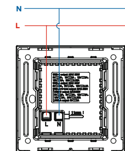
O24 2G USB Charger, Type A+C
