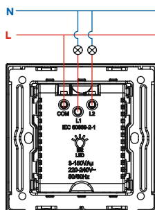
O34 LED dimmer - 1 Way operation
