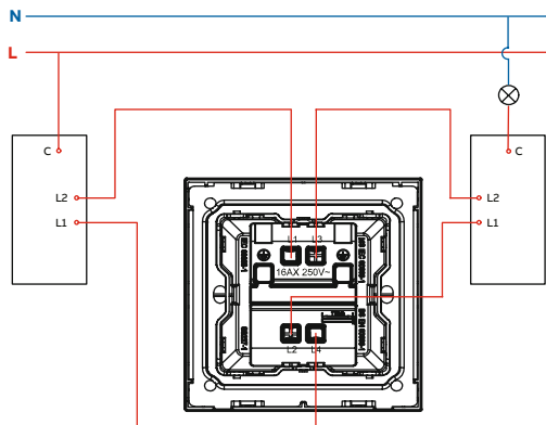
O11 1G intermediate switch
