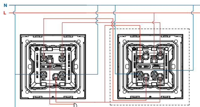
O31 DND/MUR BELL Switch (OUTDOOR)
