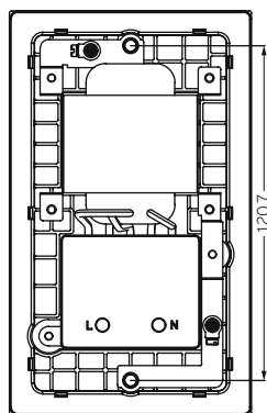
Ø6 Distance between fixing screws for Shaver socket
