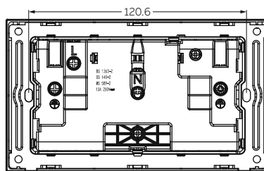
Ø4 Distance between fixing screws for 2gang frames
