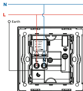
O17 1G 13 A switched socket outlet
