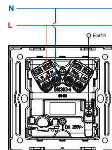
O36 Fused connection unit
