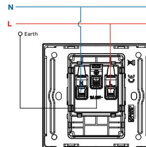
O22 1G/2G 16A Euro-American Socket with Earth
