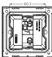
Ø2 Distance between fixing screws for 1gang frames
