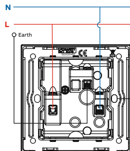
O19 1G 5 A switched socket outlet
